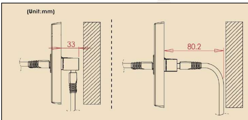
90° USB2 A to A keystone coupler (KCUAA290BK + KCUAA290WH) High performance USB2 keystone coupler ideal for use in limited space
