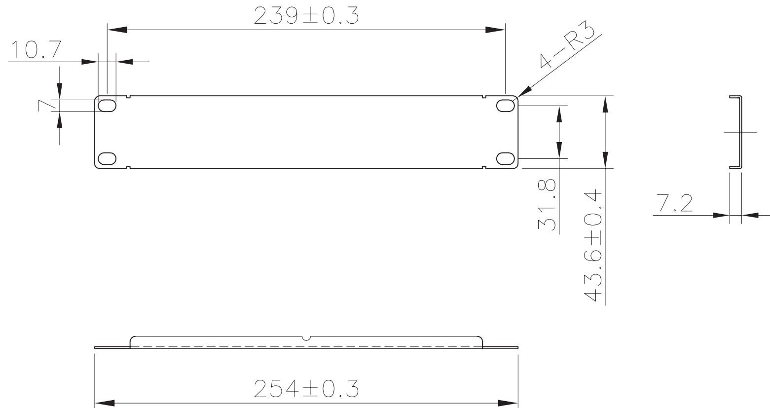
Code: MBP/10 1U Blanking Panel
